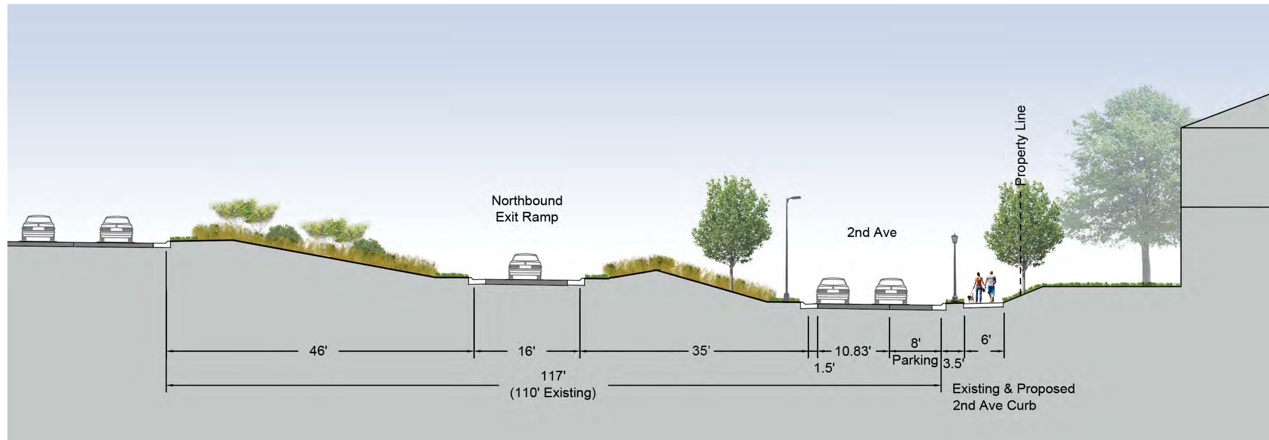
CROSS SECTION Q
