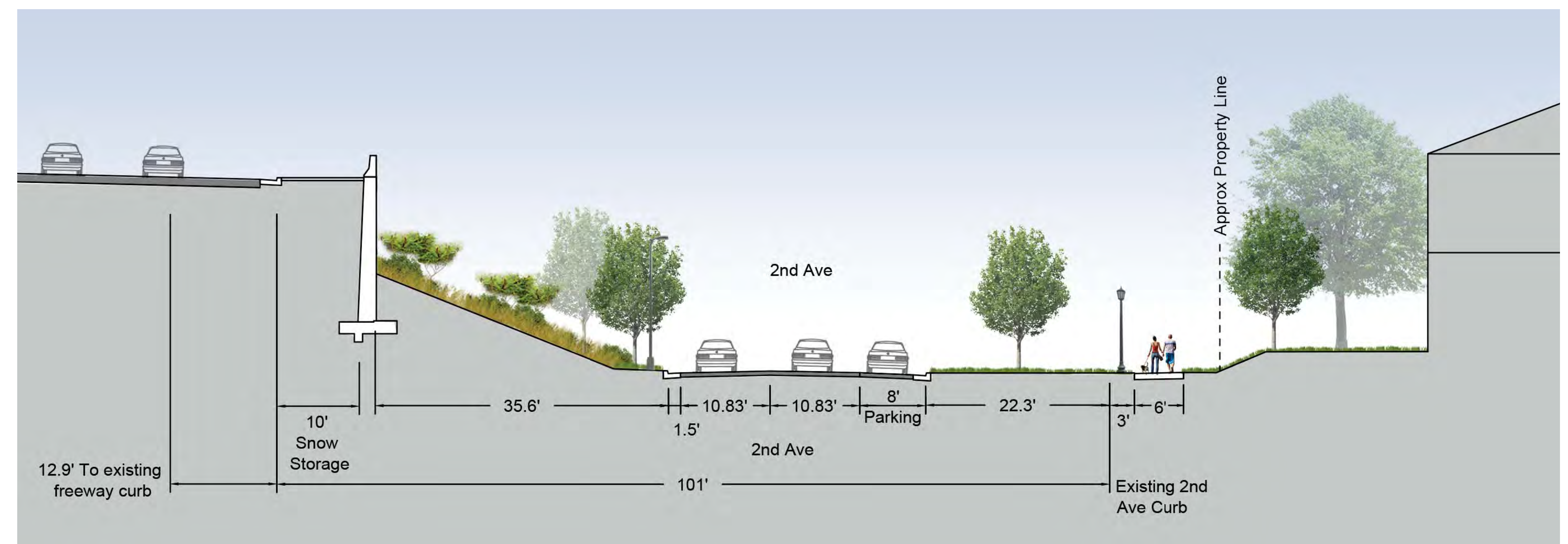
CROSS SECTION N
